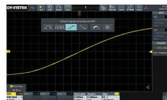
Detecting Square or Pulse Waves, the Second-level Menu Optimizes Pulse Width and Edge Timing Measurements
