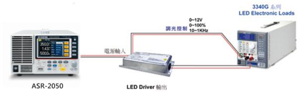
圖五 LED Driver 效率量測接線圖示
