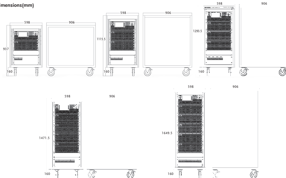
Dimensions(mm)
