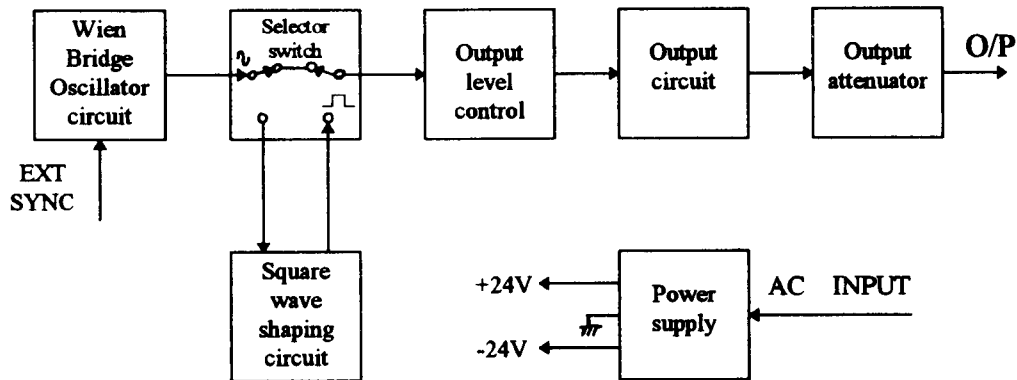
Fig.1 Block Diagram
