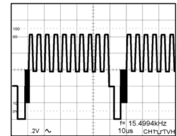
Figure 5-14(b) TV-H
