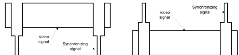
Figure 5-15 TV Signal
