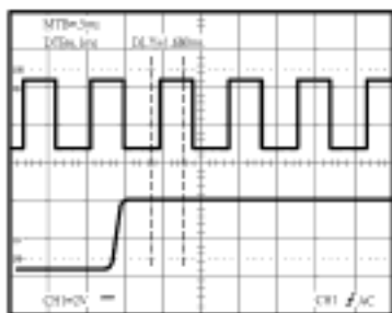
Figure 5-9 ALT Mode
