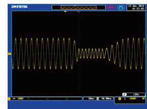
Voltage Fall
