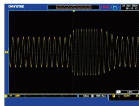
Voltage Rise
