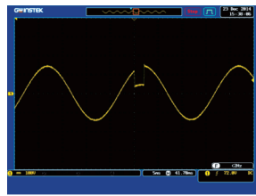
Dip
