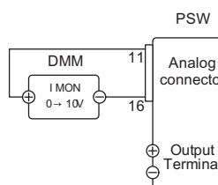
External DMM Monitoring of the Output Current
