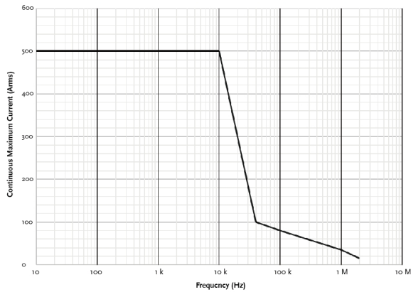
Figure 1 Derating according to frequency (For GCP-0275)
