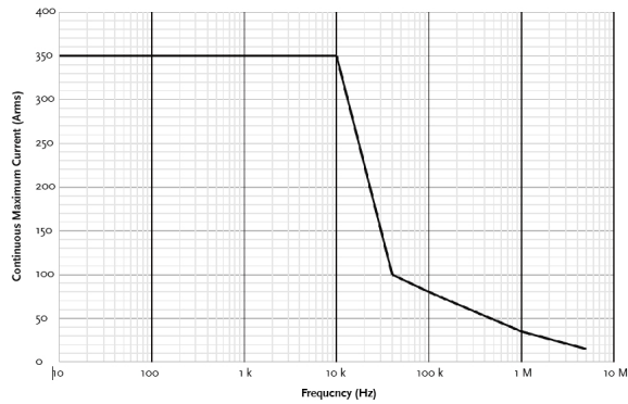
Figure 2 Derating according to frequency (For GCP-0550)
