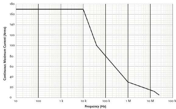
Figure 3 Derating according to frequency (For GCP-2525)
