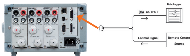
DA12 Interface Mechanism
