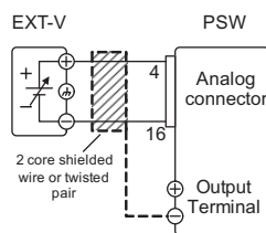
External Voltage Control of the Voltage Output
