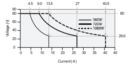
PSW 80V Series Operating Area
