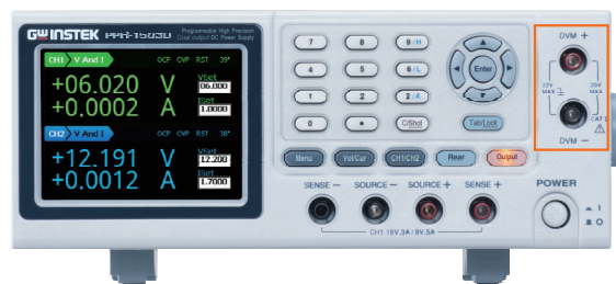
DVM Input for PPH-15xxD
