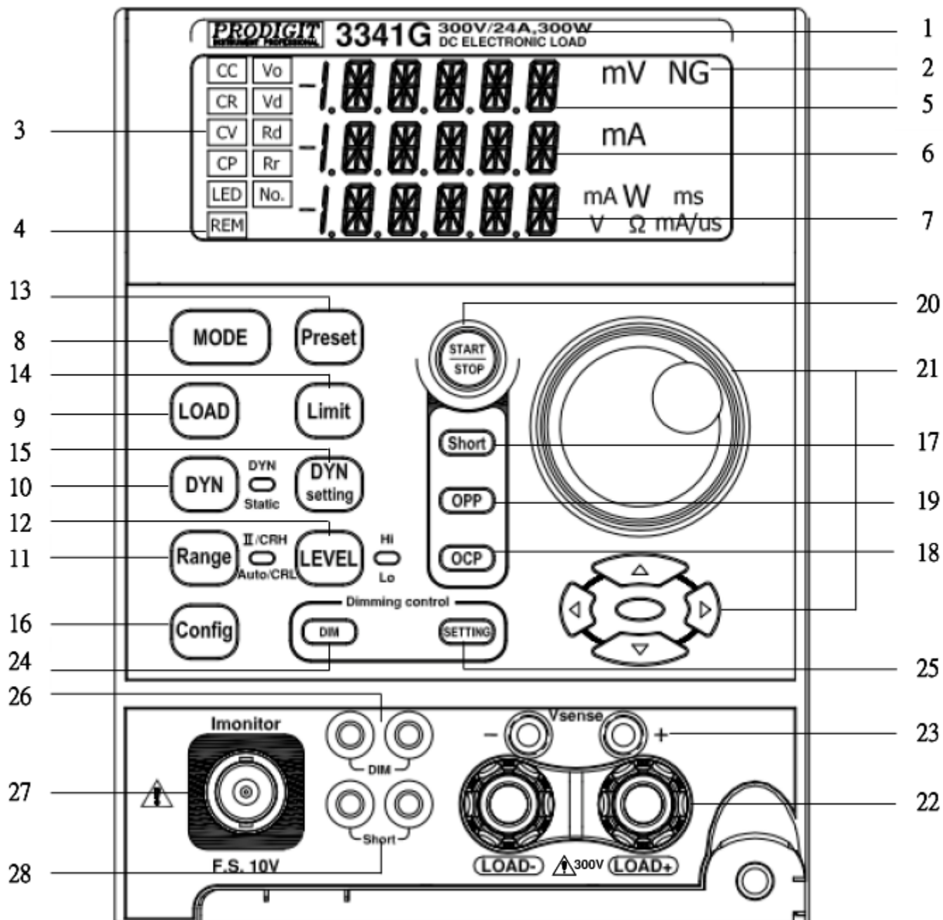
Fig 3-1 Front panel of 3341G plug-in module
