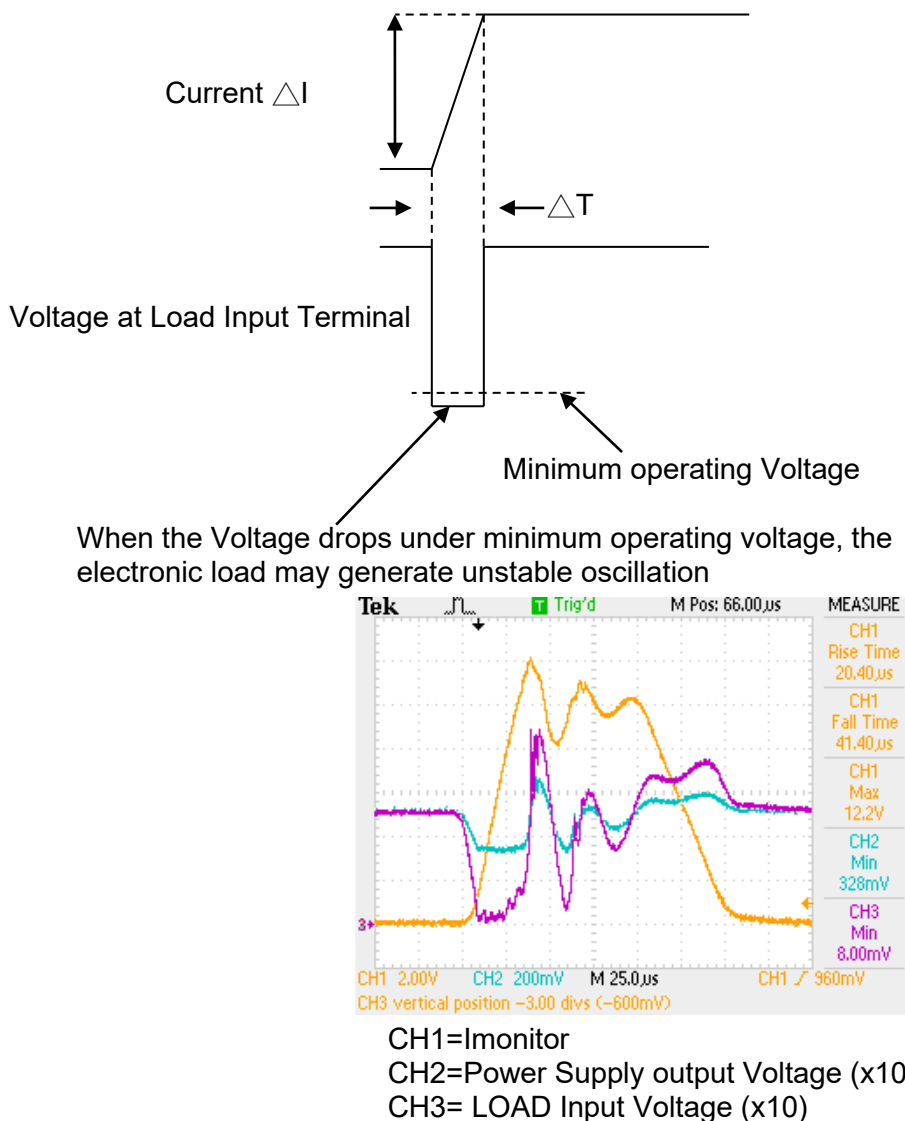
Fig 2-4 Waveform example: Generate unstable oscillation
