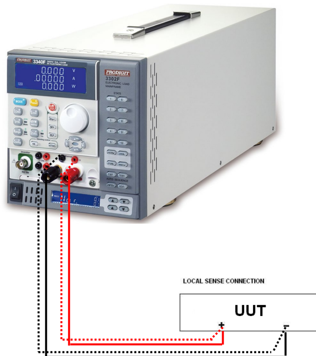
Fig 4-2 Remote voltage sense connections
