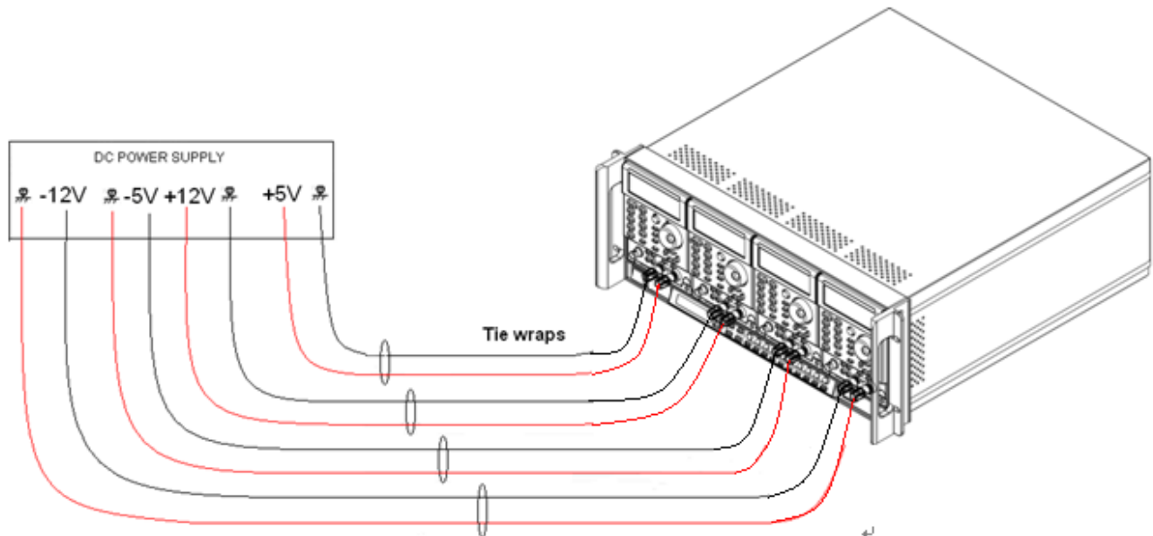
Fig 4-13 Connection between 3341G series plug-in load and multiple output power supply
