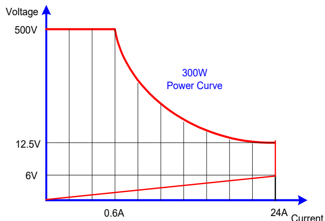
Fig 1-3 3343G 500V/24A/300W power contour
