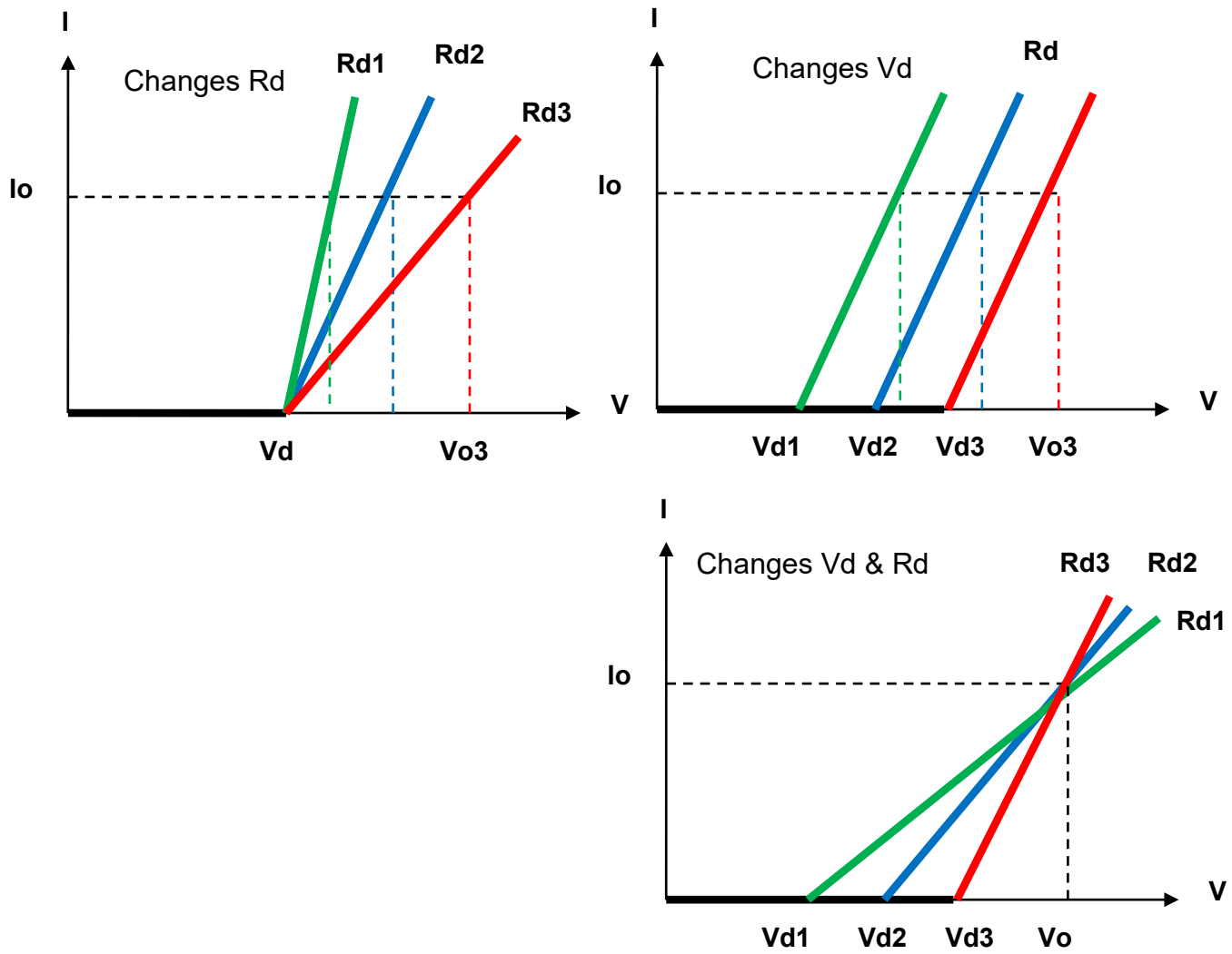
Fig 4-12 LED MODE operation mode of the application
