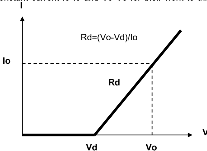
Fig 1-8 LED mode characteristics
