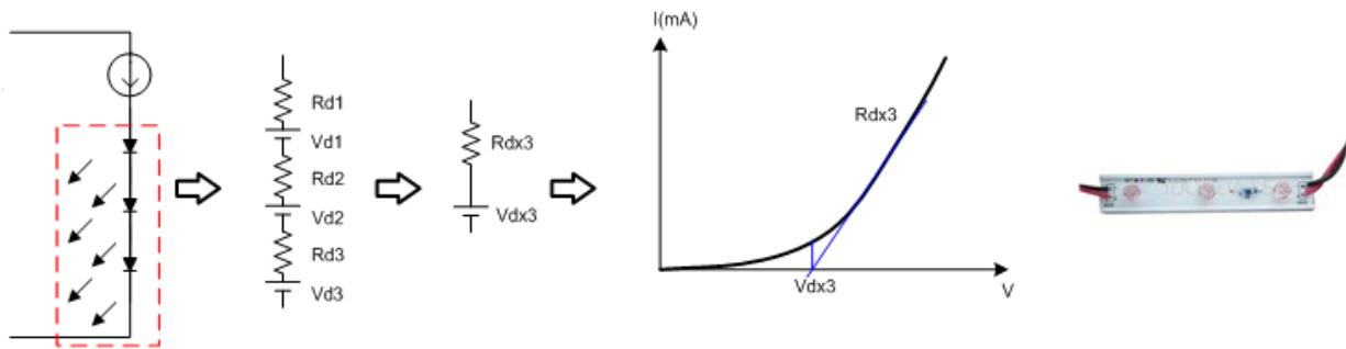
Fig 4-10 3 LED cascading connection equivalent circuit and characteristic curve
