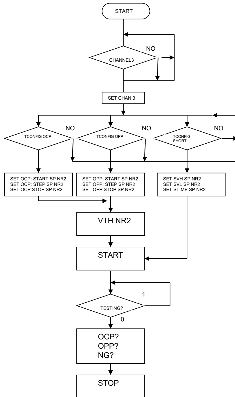
Fig 4-16 3341G series electronic load OCP, OPP, SHORT operation flow chart
