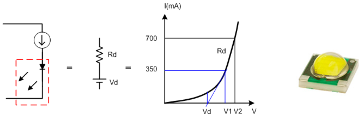
Fig 4-8 LED's equivalent circuit and characteristic curve
