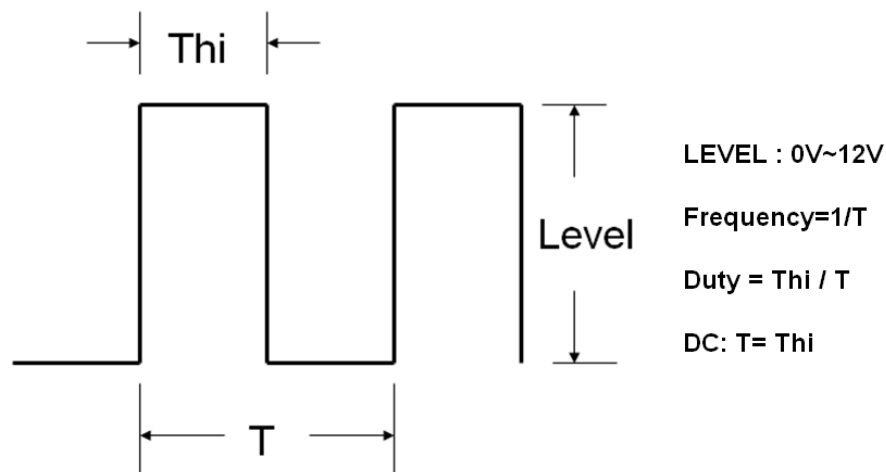
Fig 3-3 3341G Series Electronic Load DIM
