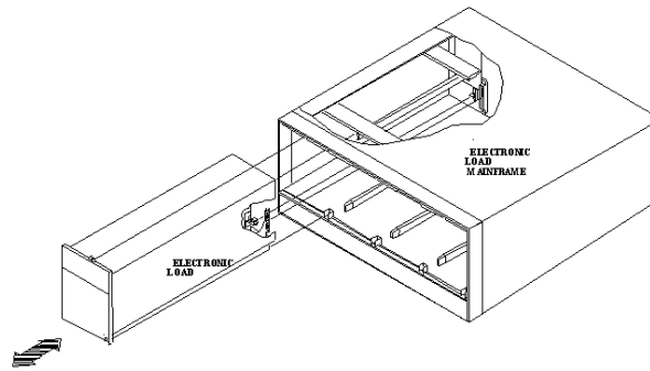
Fig 2-2 Plug-in installation and removal
