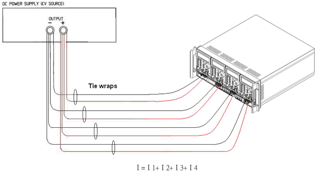
Fig 4-14 3341G series plug-in module parallel operation
