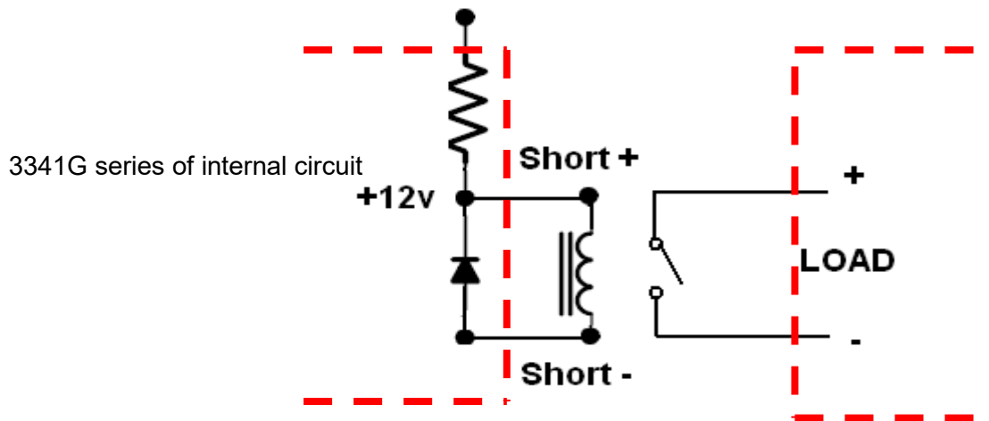
Fig 4-17 short test connection
