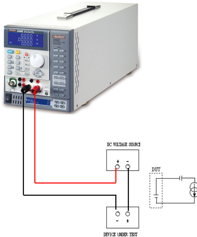
Fig 4-15 Zero-Volt loading connection
