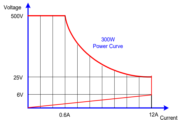
Fig 1-2 3342G 500V/12A/300W power contour
