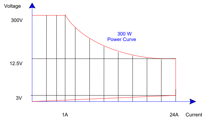
Fig 1-1 3341G 300V/24A/300W power contour
