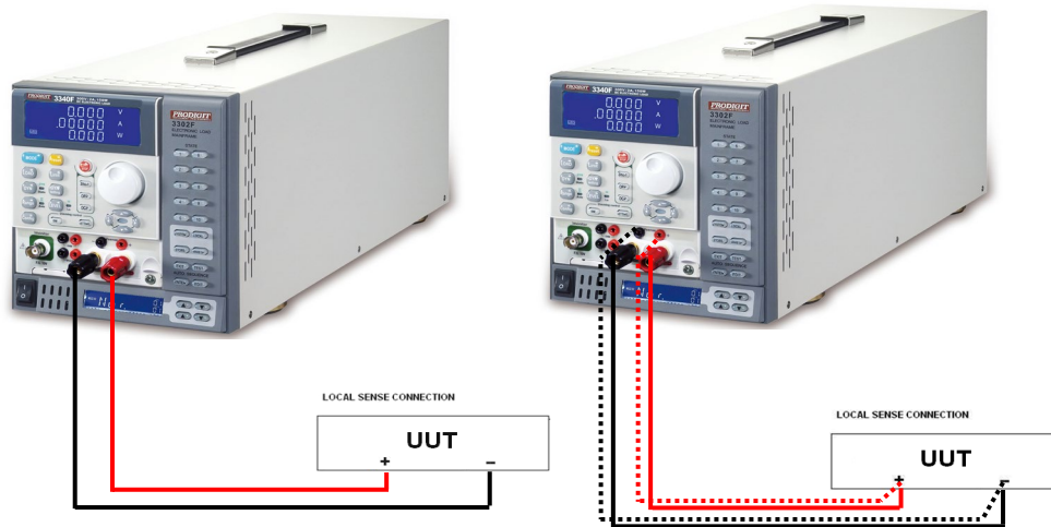
Fig 3-2 typical connection of 3341G series load module
