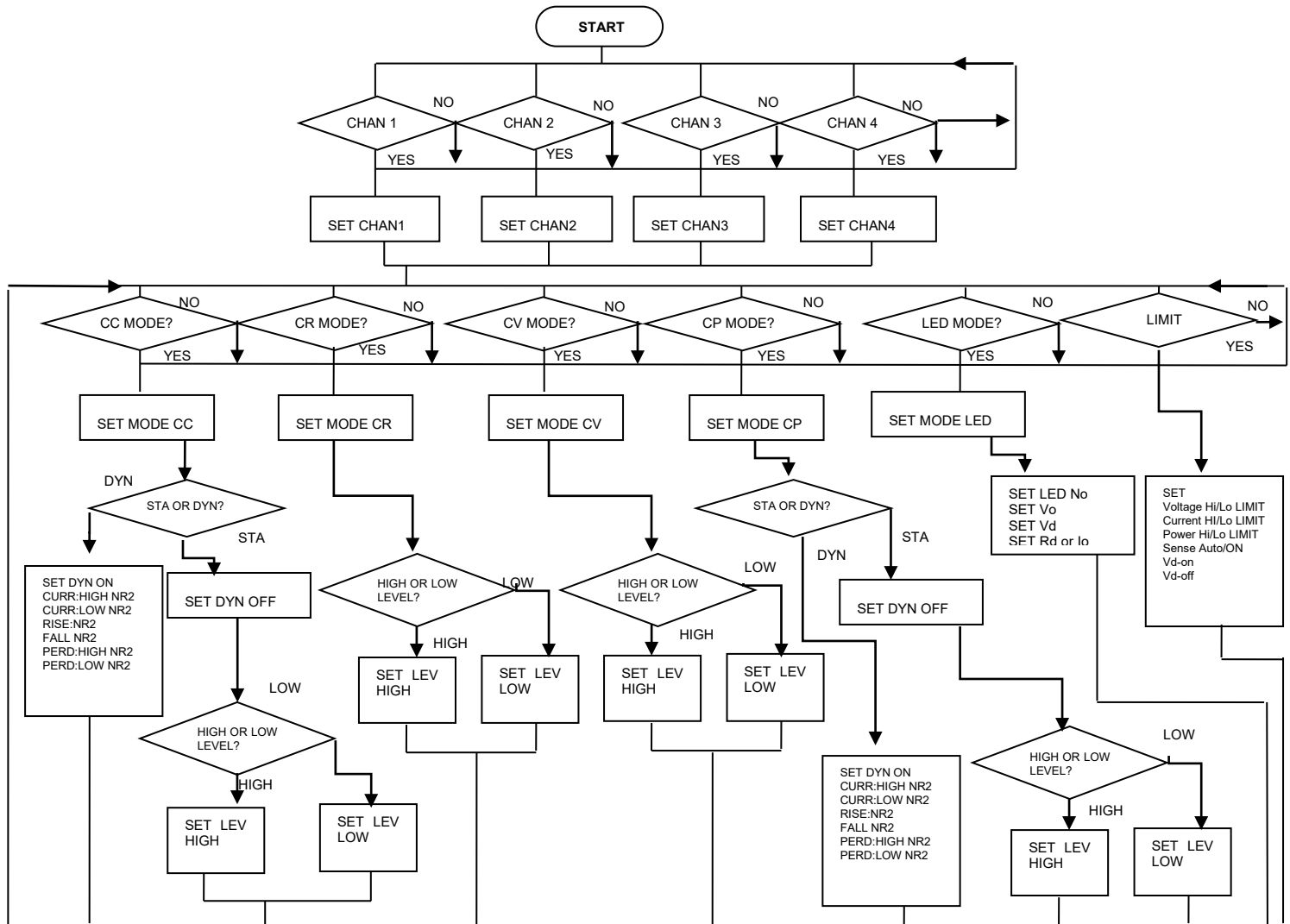
Fig 2-3 3341G series electronic load module load condition setting flow chart
