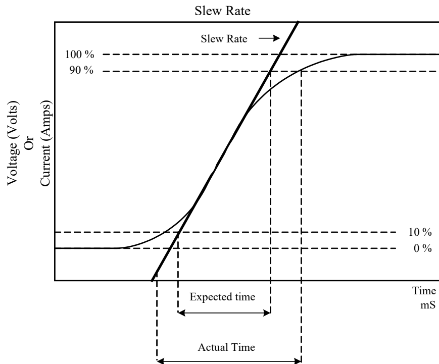
Fig 1-10 Rise Time Transition Limitation
