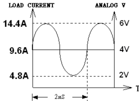
Fig 3-7 Analog programming load current in CC mode operation
