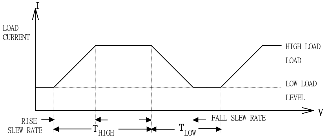
Fig 1-9 Dynamic Wave form
