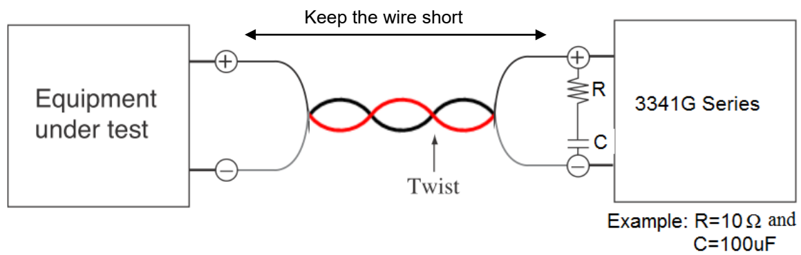
Fig 2-5 Length of wiring
