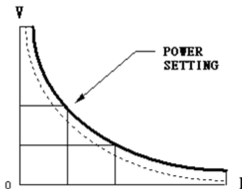
Fig 1-7 Constant Power mode
