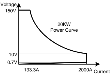
PEL-5020C-150-2000 power contour
