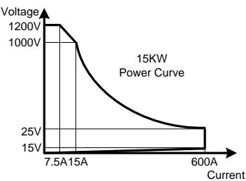
PEL-5015C-1200-600 power contour
