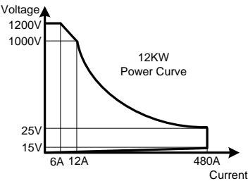
PEL-5012C-1200-480 power contour
