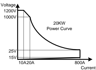
PEL-5020C-1200-800 power contour
