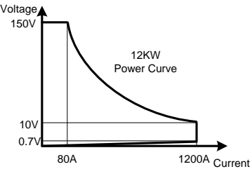
PEL-5012C-150-1200 power contour
