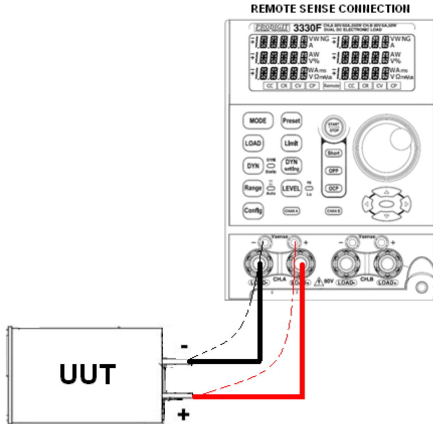
Fig 4-2 Remote voltage sense connections
