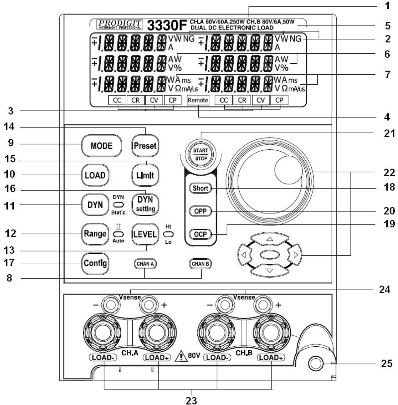
Fig 3-1 Front panel of 3330F plug-in module
