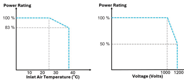
Curve on the Brand C Catalog, Left is The Temperature De-rating Curve; Right is The Voltage De-rating Curve.
