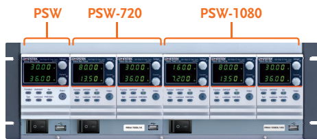
Rack Mount Kit GRA-410-J (JIS)
